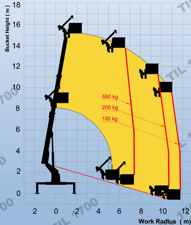
Outrigger extension MAX 3.5(m)
