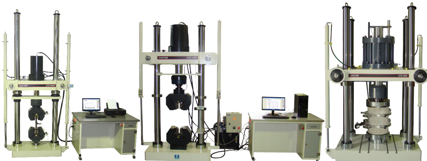
STD-600B With Pneumatic Wedge Grips
