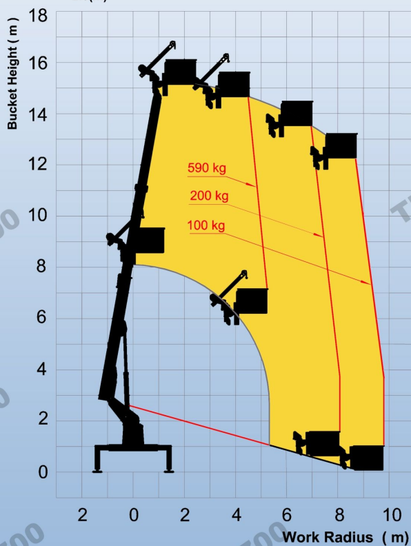
Outrigger extension MID 2.8(m)
