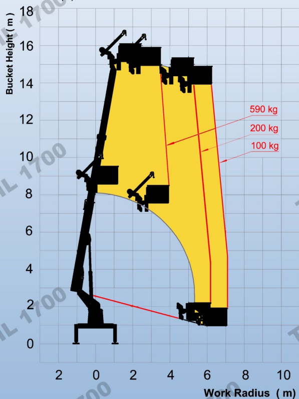
Outrigger extension MIN 2.1(m)
